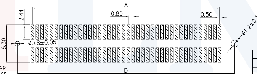
Recommended P.C.B Layout (Top Side)
