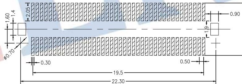
Recommended P.C.B Layout(Top Side) (PCB BOARD TOLERANCE±0.05)
