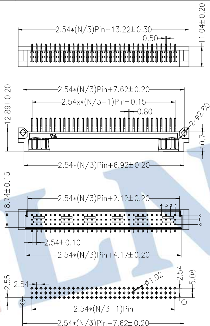
Recommended P.C.B Layout(Top Side) (PCB BOARD TOLERANCE \pm 0.05 )
