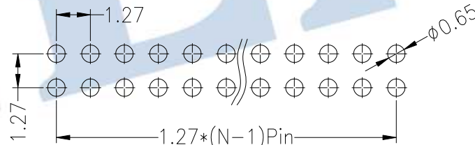
Recommended P.C.B Layout(Top Side) (PCB BOARD TOLERANCE± 0.05)
