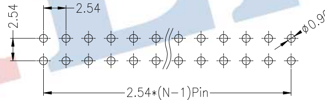
Recommended P.C.B Layout(Top Side) (PCB BOARD TOLERANCE±0.05)
